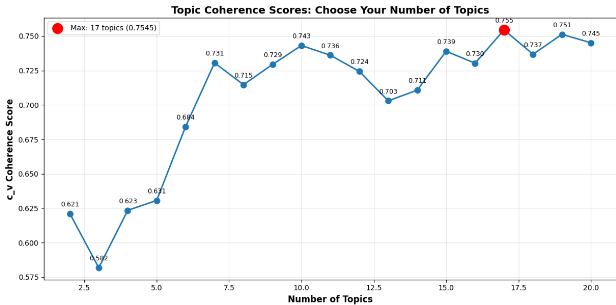
Figure AF01 – Coherence scores for topic models from two to 20
