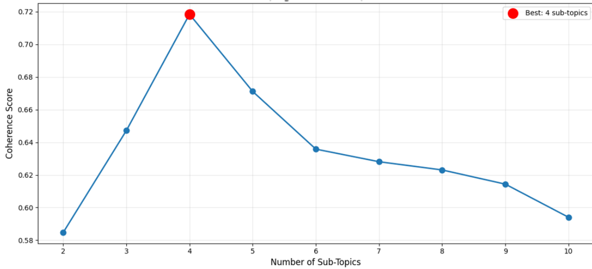
Figure AF03 – Coherence scores for sub-topic models from two to 10
